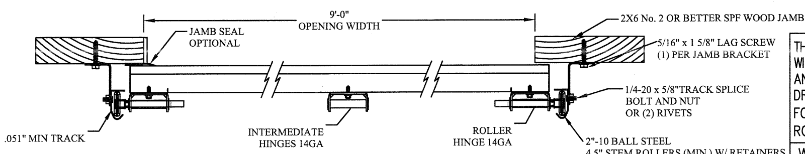
2" BRACKET MOUNT TO WOOD JAMB DETAIL
