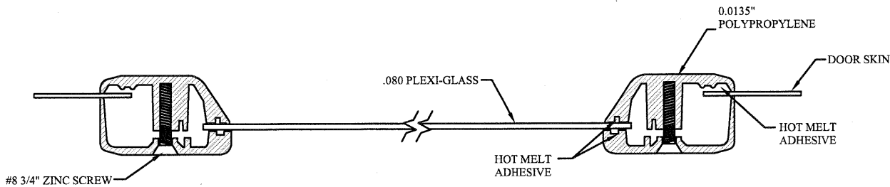
SECTION C-C 24" X 12" WINDOW DETAIL W/ .080 PLEXI-GLASS N.T.S.
