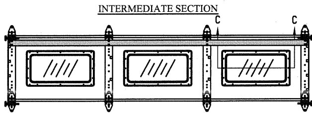
OPTIONAL GLAZED SECTION W/ 24" X 12" WINDOWS AND STRUT LAYOUT N.T.S.
